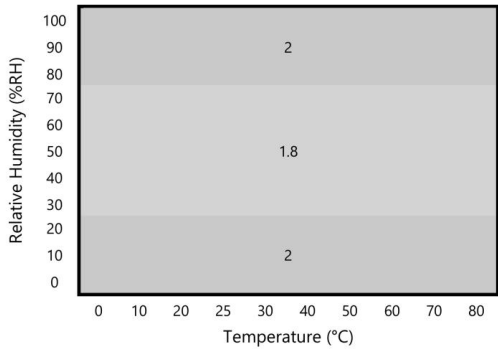
4. Typical RH accuracy corresponding to the temperature.
