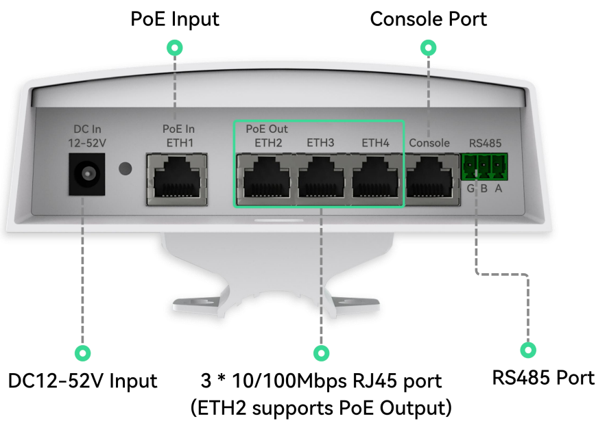
Left View
