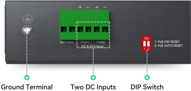
Left View
